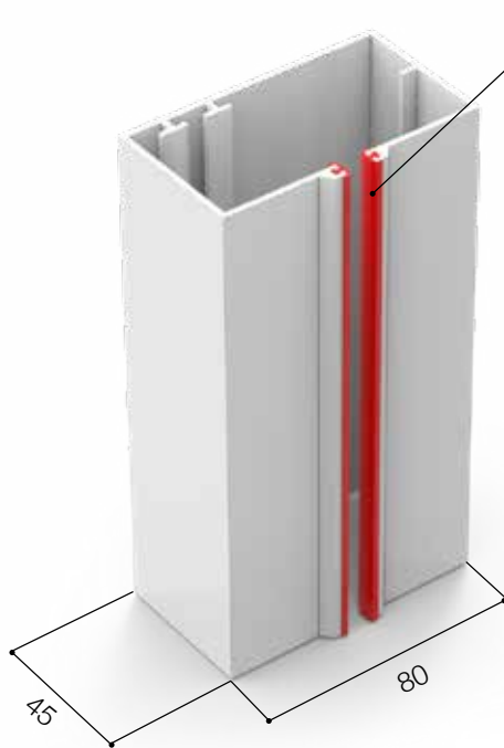
Guida standard - cod. 965
